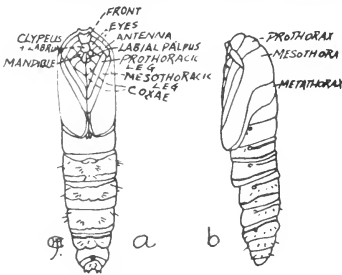
Fig. 505. Sthenopsis thule Stkr. a, ventral aspect; b, lateral aspect.
